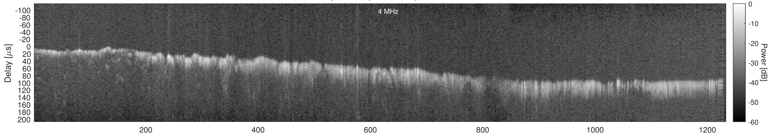
Orbit 6249, Window, Channel 2, Chapman
