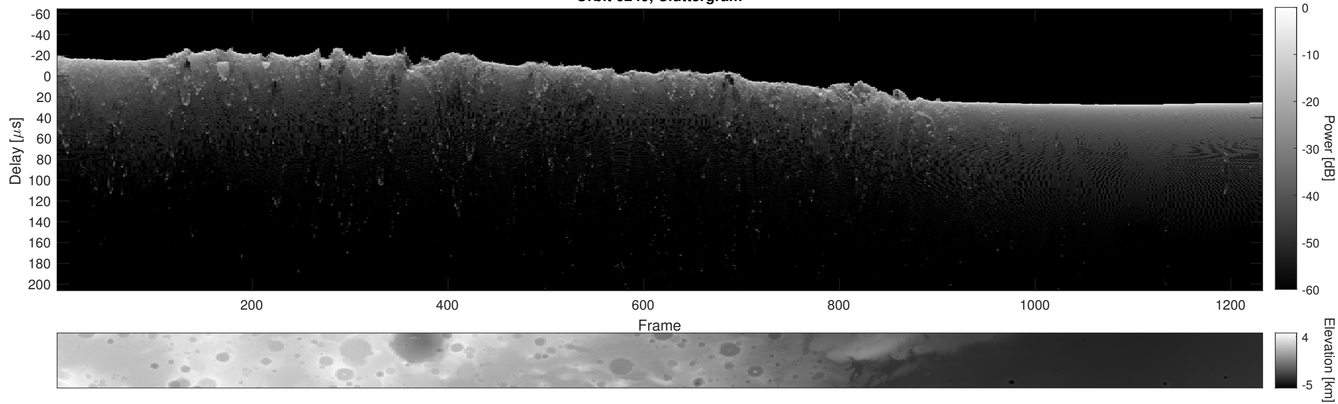
Orbit 6249, Cluttergram
