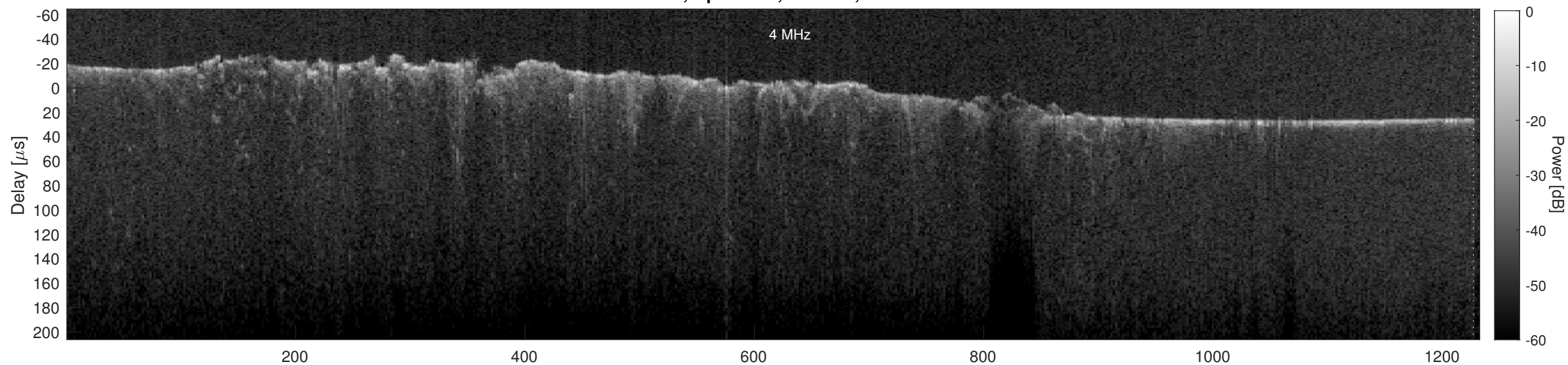
Orbit 6249, Cluttergram
