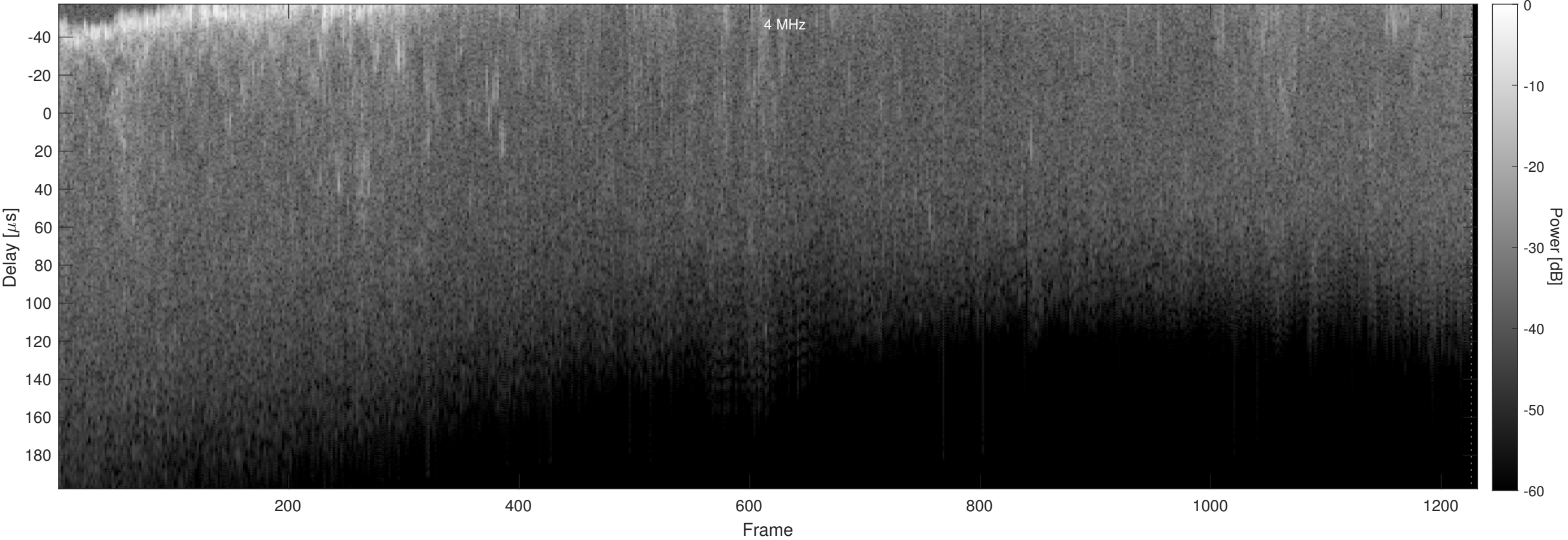
Orbit 6251, Chapman, Window, Channel 2
