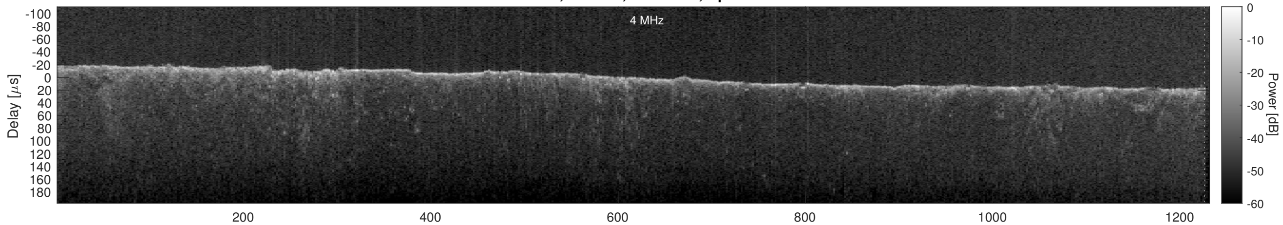
Orbit 6251, Cluttergram
