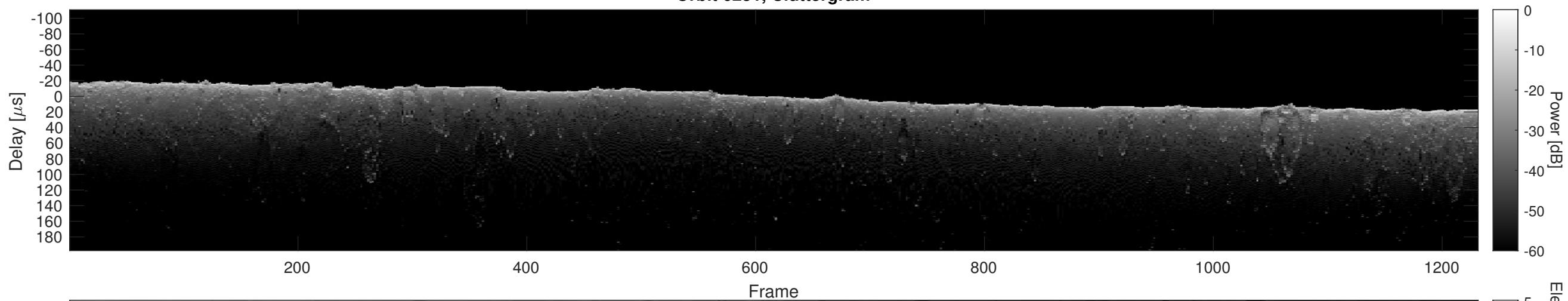
Orbit 6251, Cluttergram
