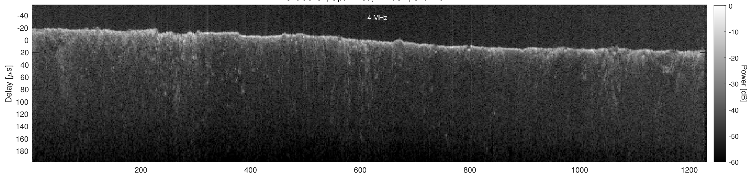
Orbit 6251, Cluttergram
