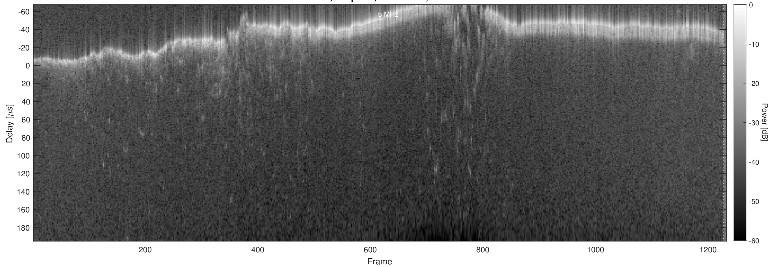
Orbit 6252, Chapman, No Window, Channel 2
