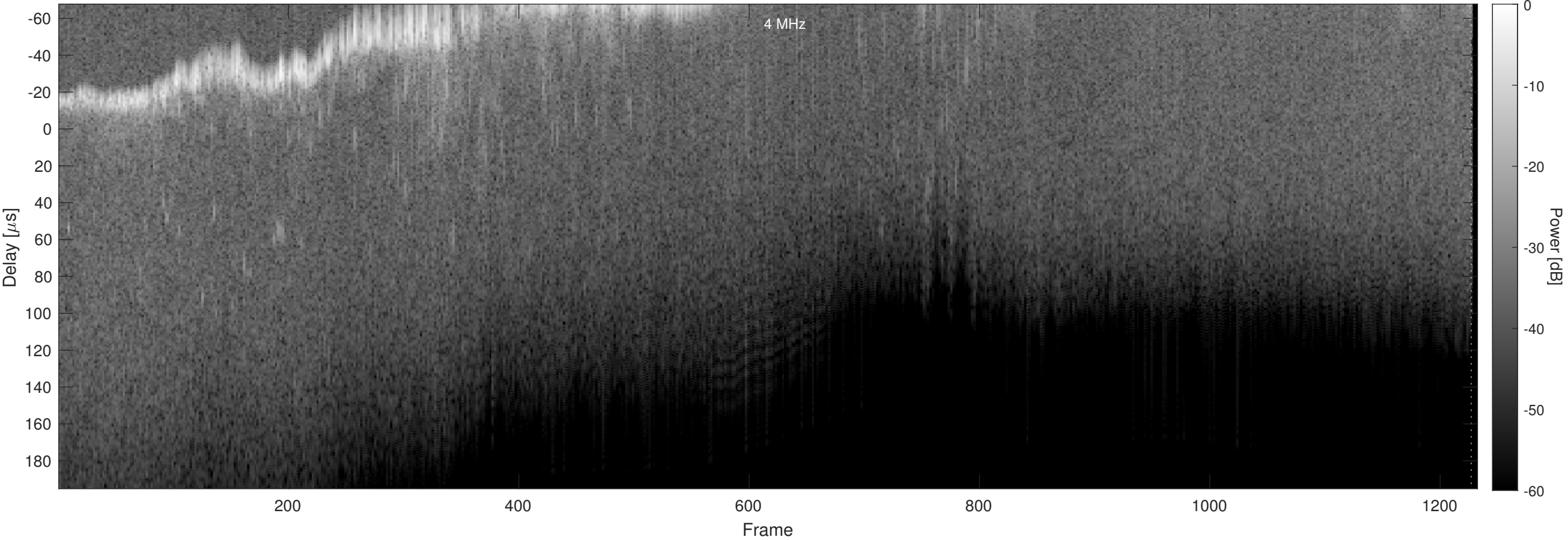
Orbit 6252, Chapman, Window, Channel 2
