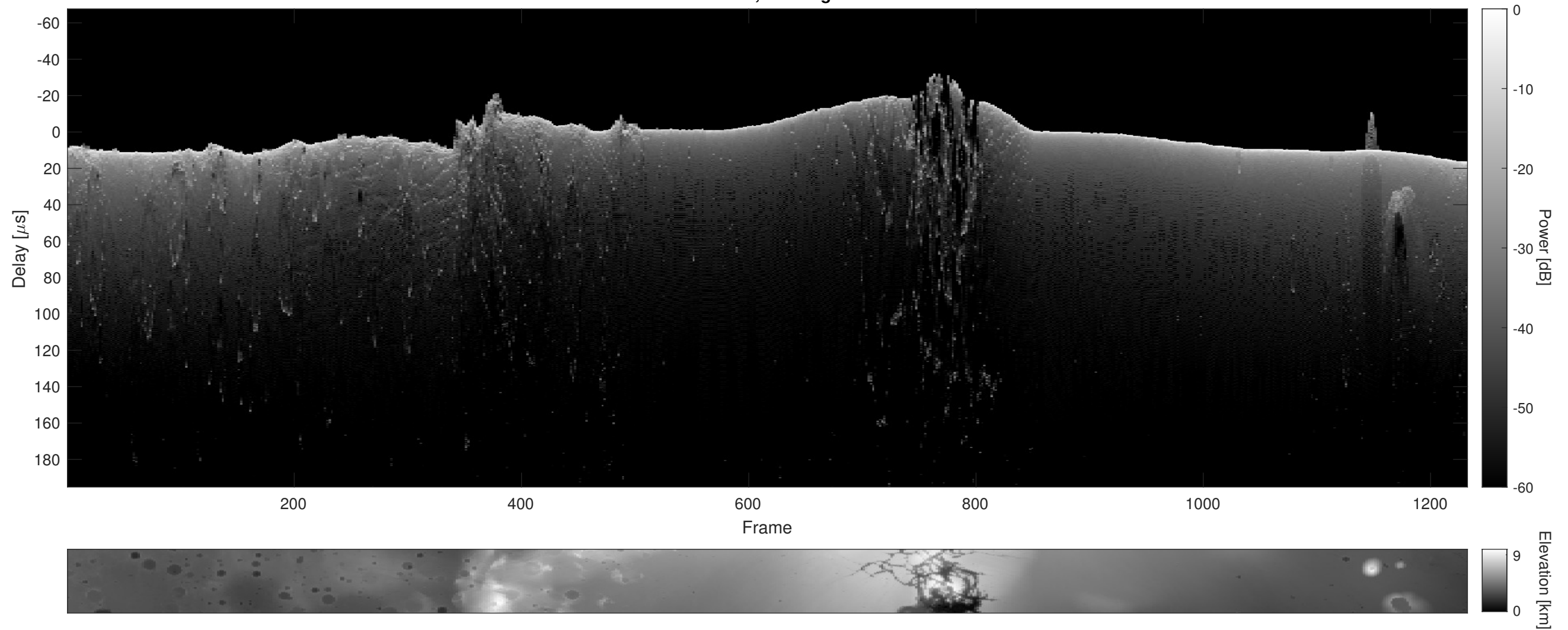
Orbit 6252, Cluttergram
