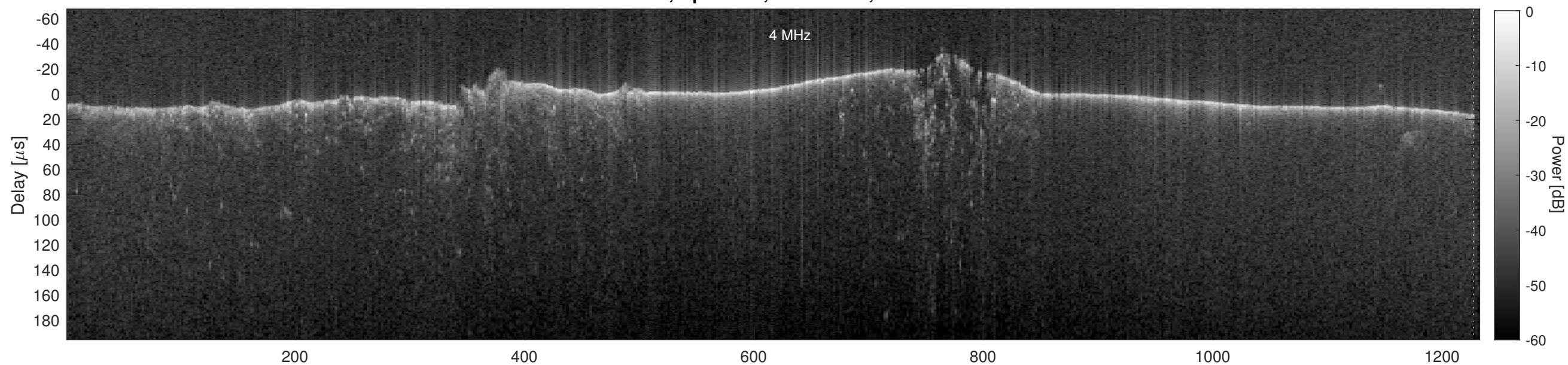
Orbit 6252, Cluttergram
