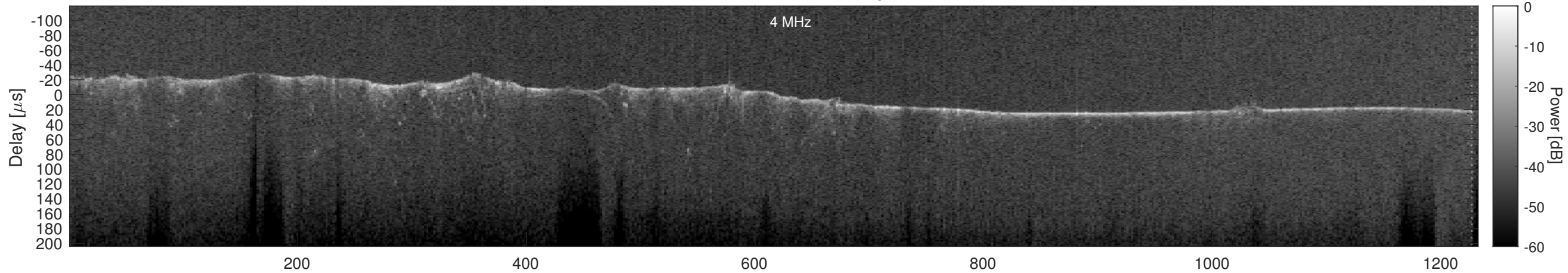
Orbit 6253, Cluttergram
