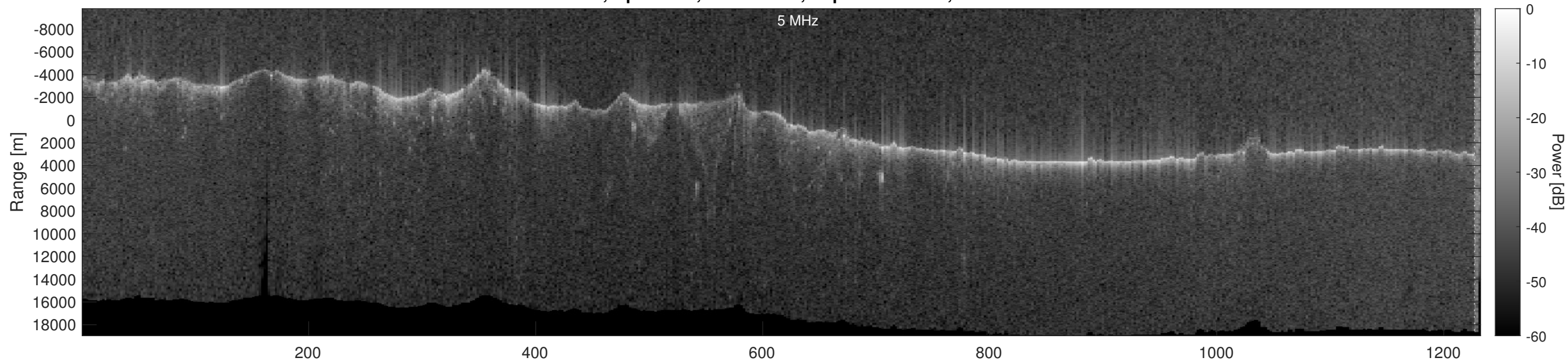
Orbit 6253, Optimized, No Window, Depth-Corrected, Channel 2
