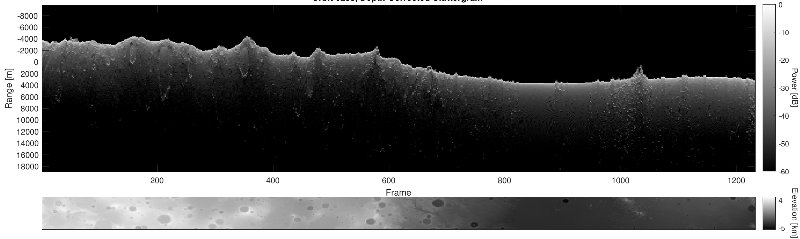
Orbit 6253, Depth-Corrected Cluttergram
