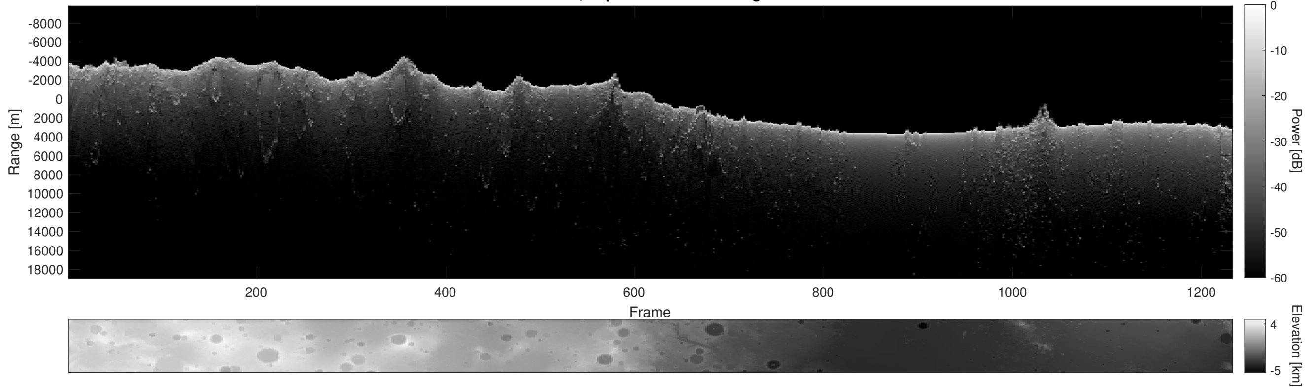
Orbit 6253, Depth-Corrected Cluttergram
