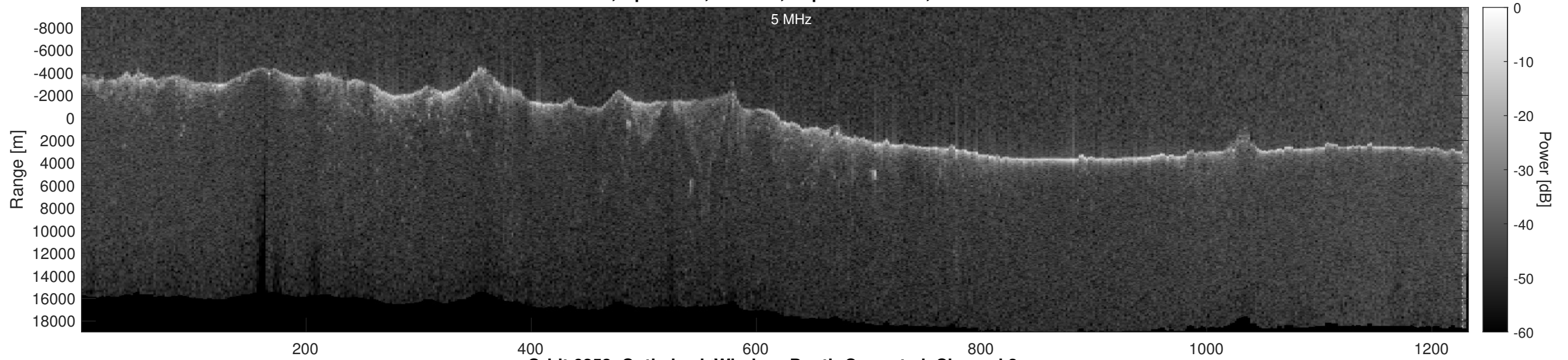
Orbit 6253, Optimized, Window, Depth-Corrected, Channel 2
