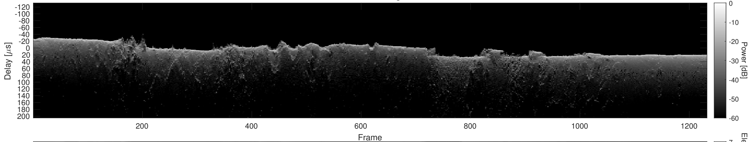
Orbit 6255, Cluttergram
