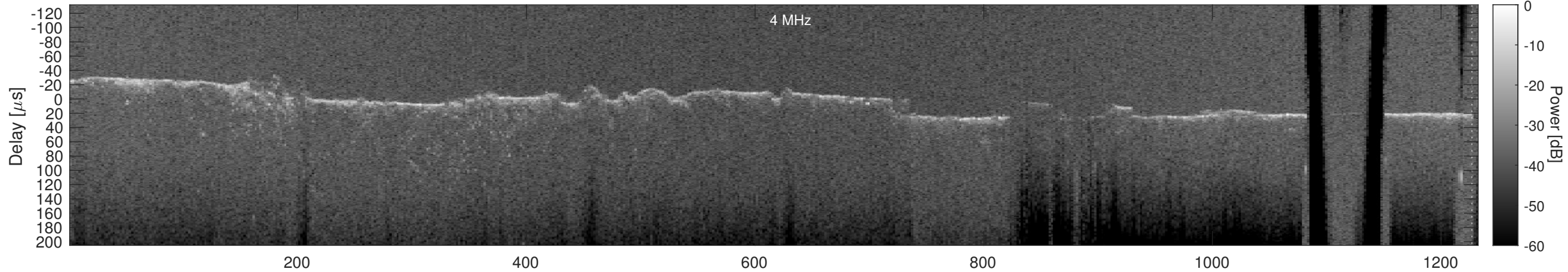
Orbit 6255, Cluttergram
