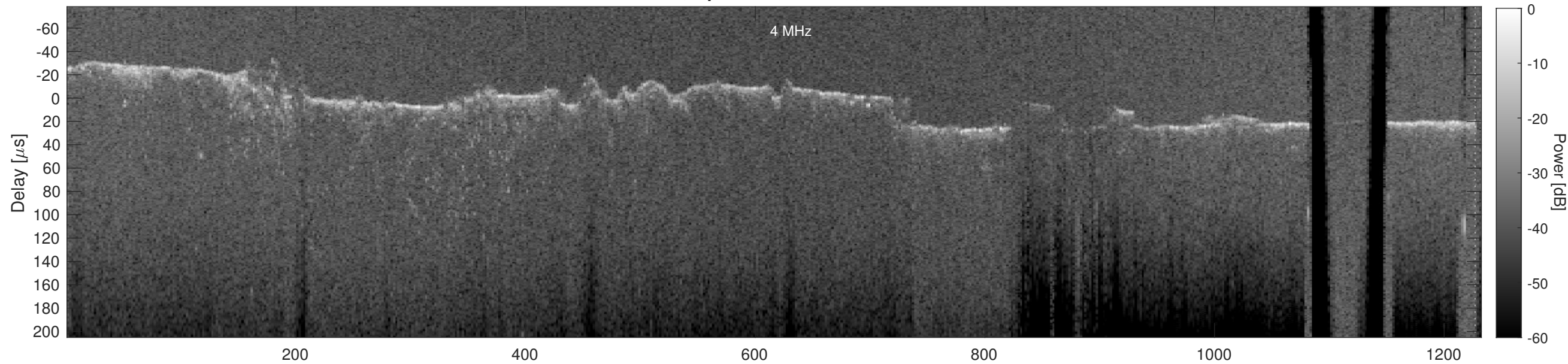
Orbit 6255, Cluttergram
