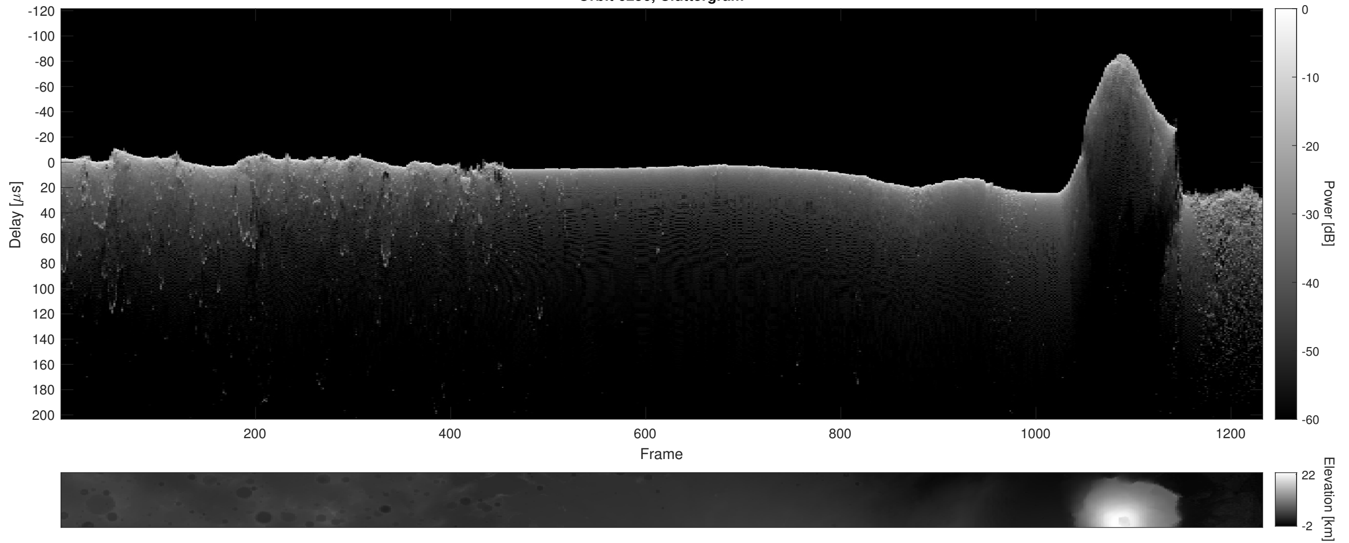
Orbit 6256, Cluttergram
