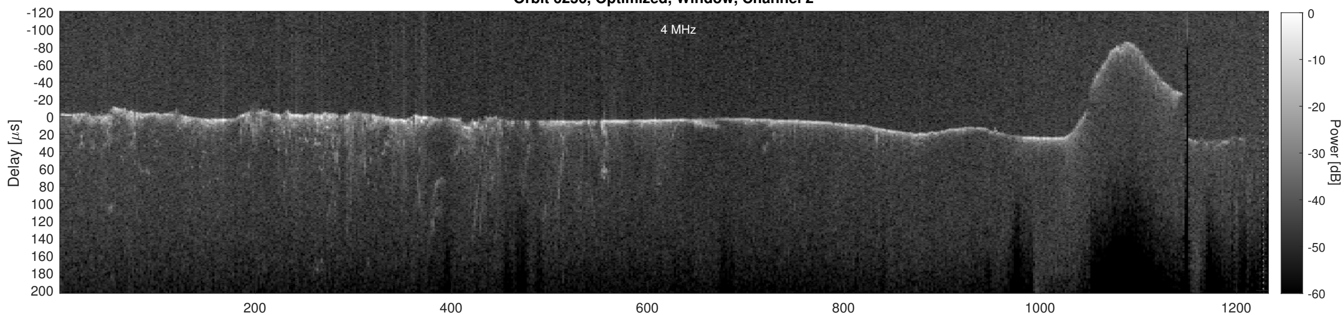
Orbit 6256, Cluttergram
