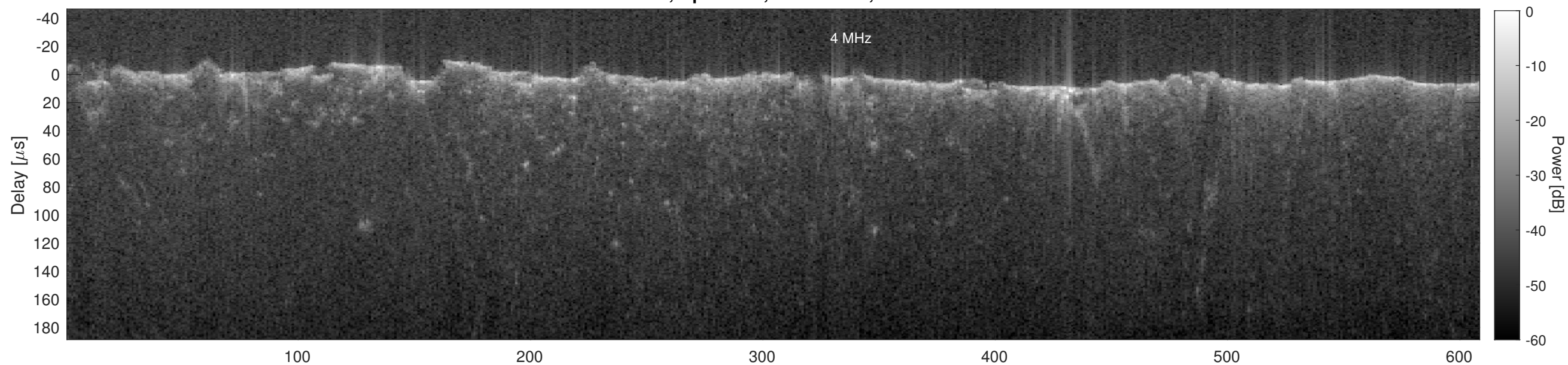
Orbit 6257, Cluttergram
