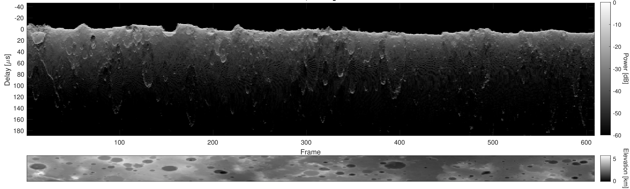
Orbit 6257, Cluttergram
