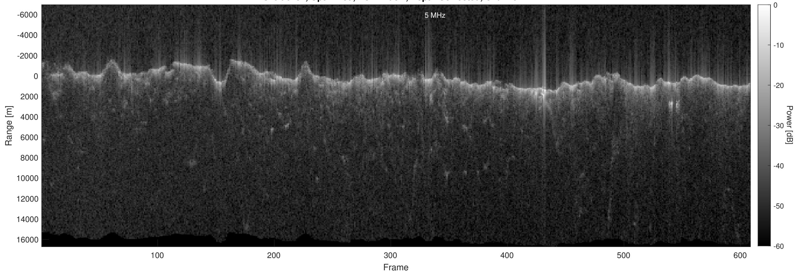
Orbit 6257, Optimized, No Window, Depth-Corrected, Channel 2
