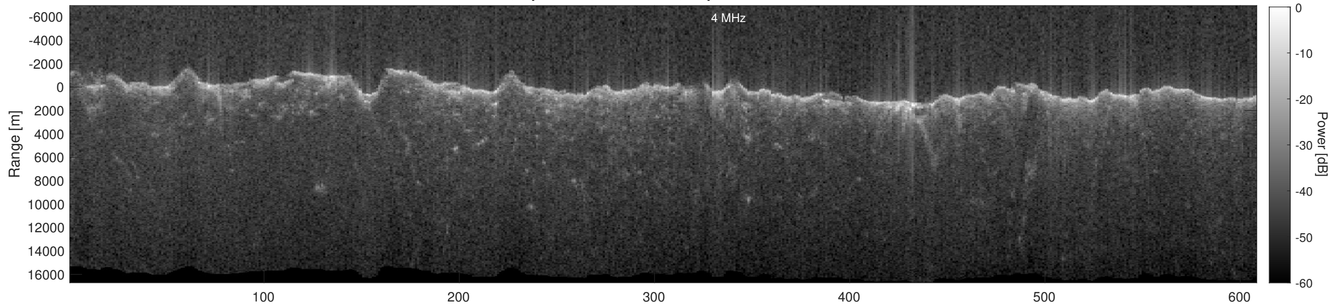
Orbit 6257, Depth-Corrected Cluttergram
