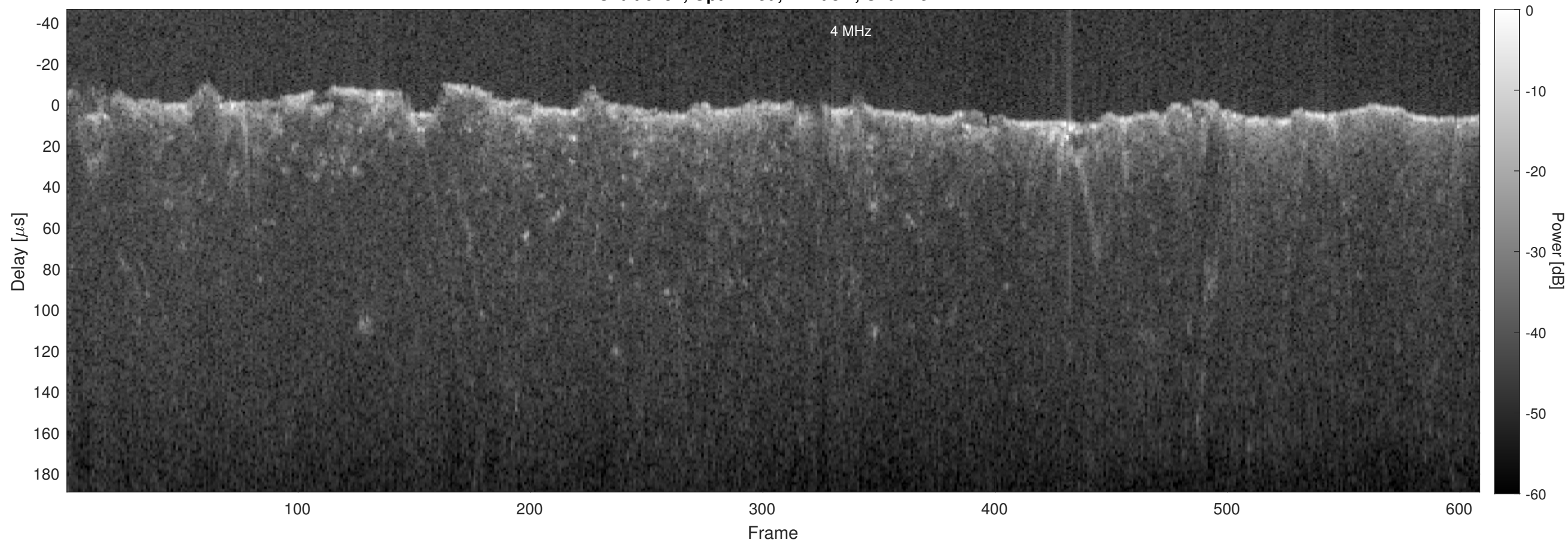
Orbit 6257, Optimized, Window, Channel 2
