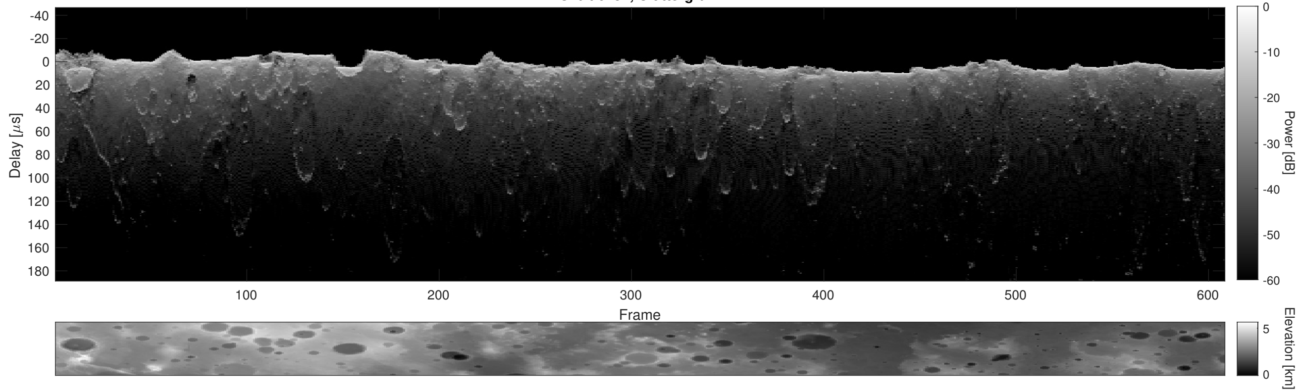
Orbit 6257, Cluttergram
