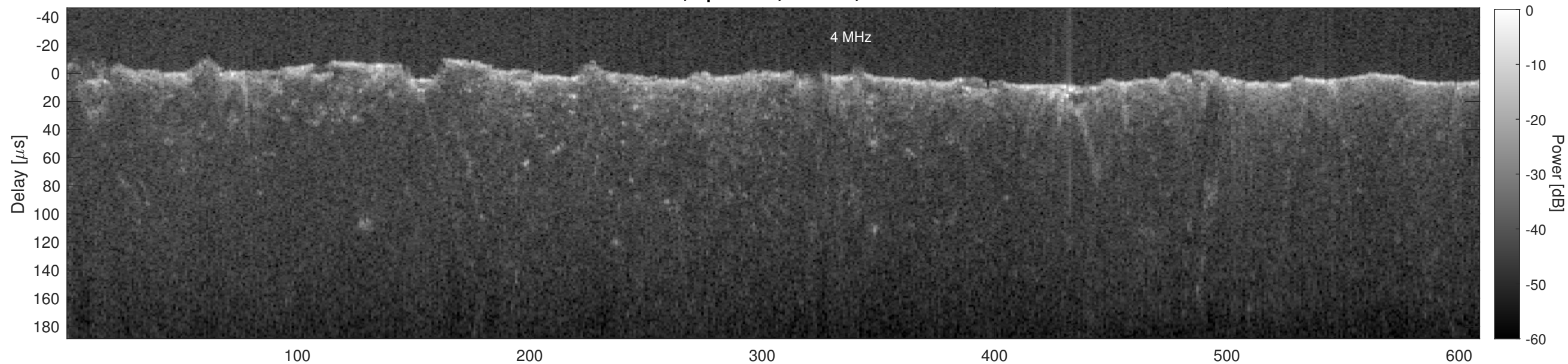
Orbit 6257, Cluttergram
