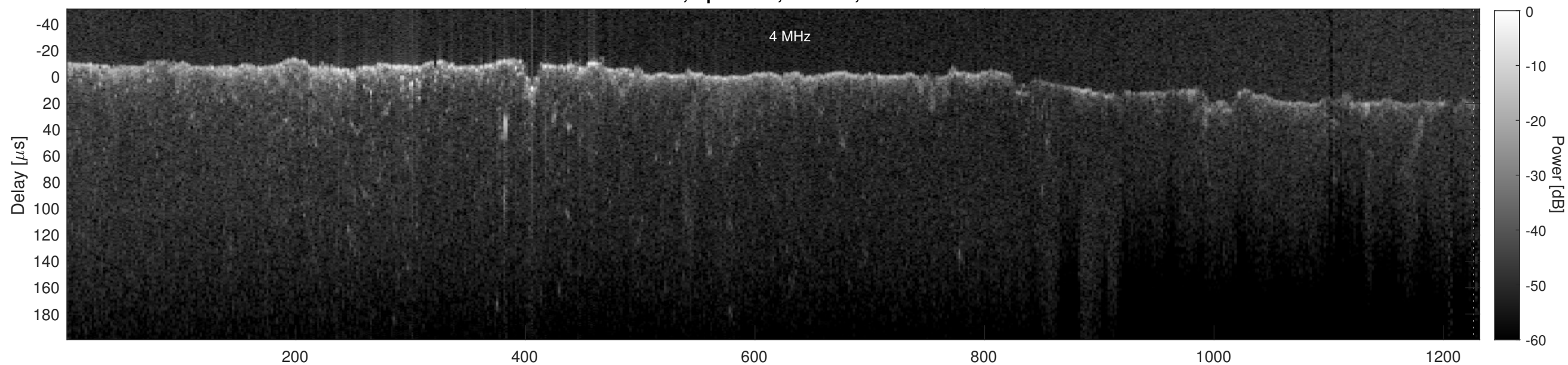
Orbit 6258, Cluttergram
