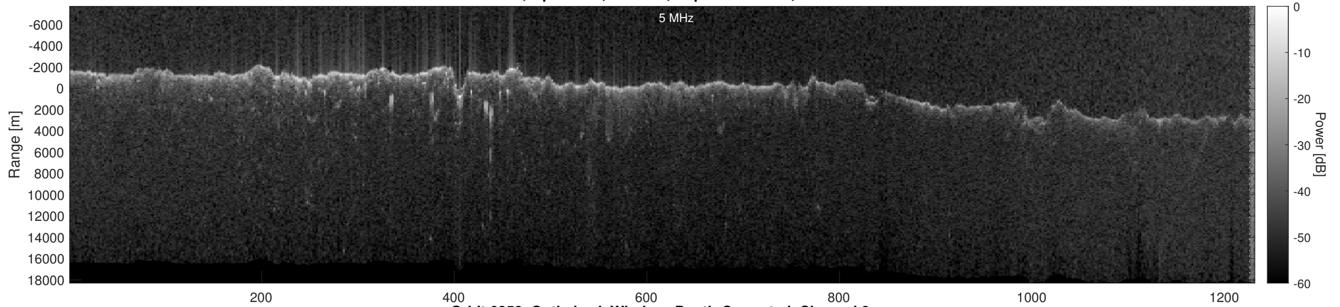
Orbit 6258, Optimized, Window, Depth-Corrected, Channel 2
