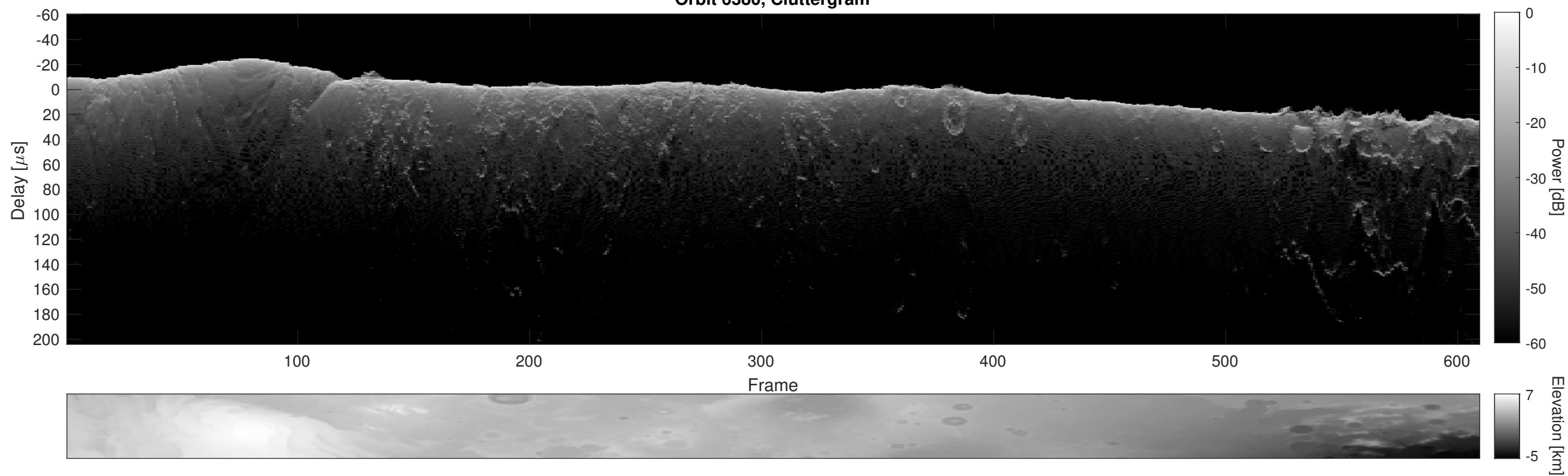
Orbit 6380, Cluttergram
