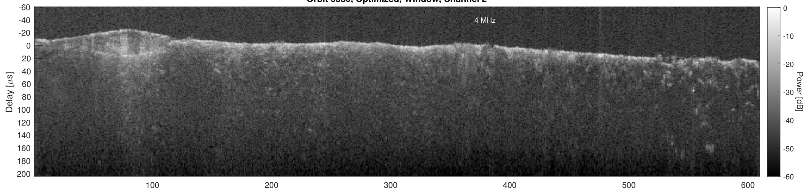
Orbit 6380, Cluttergram
