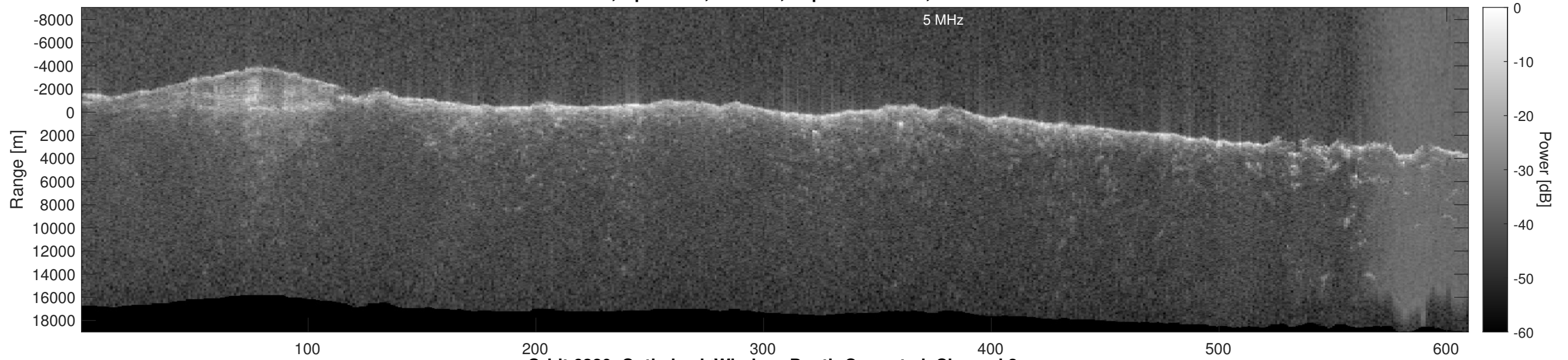
Orbit 6380, Optimized, Window, Depth-Corrected, Channel 2
