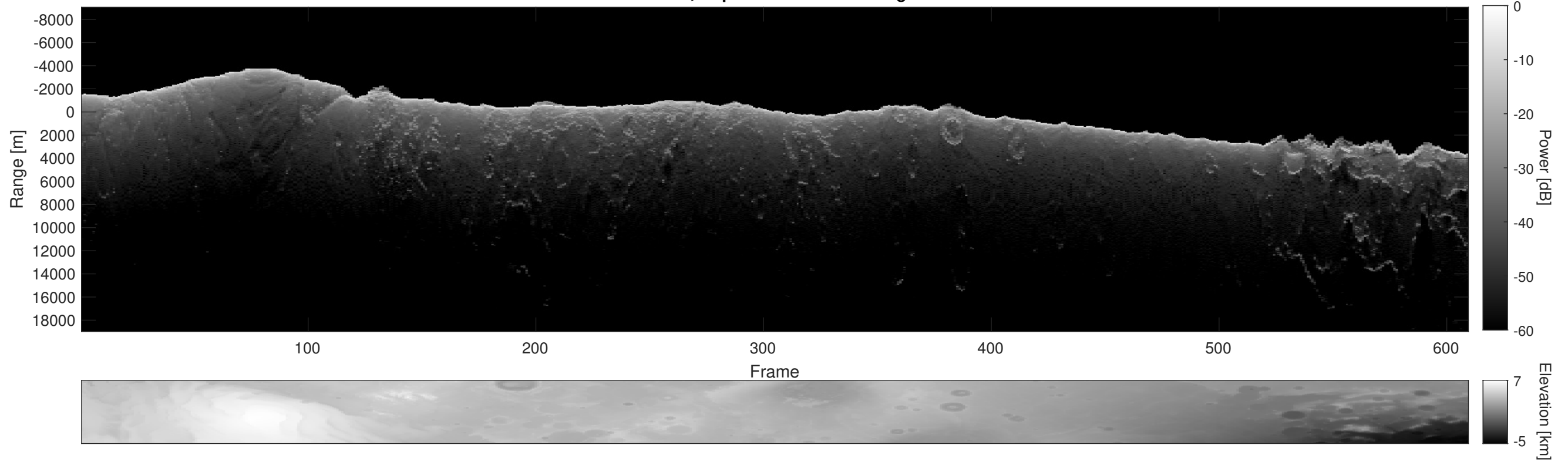
Orbit 6380, Depth-Corrected Cluttergram
