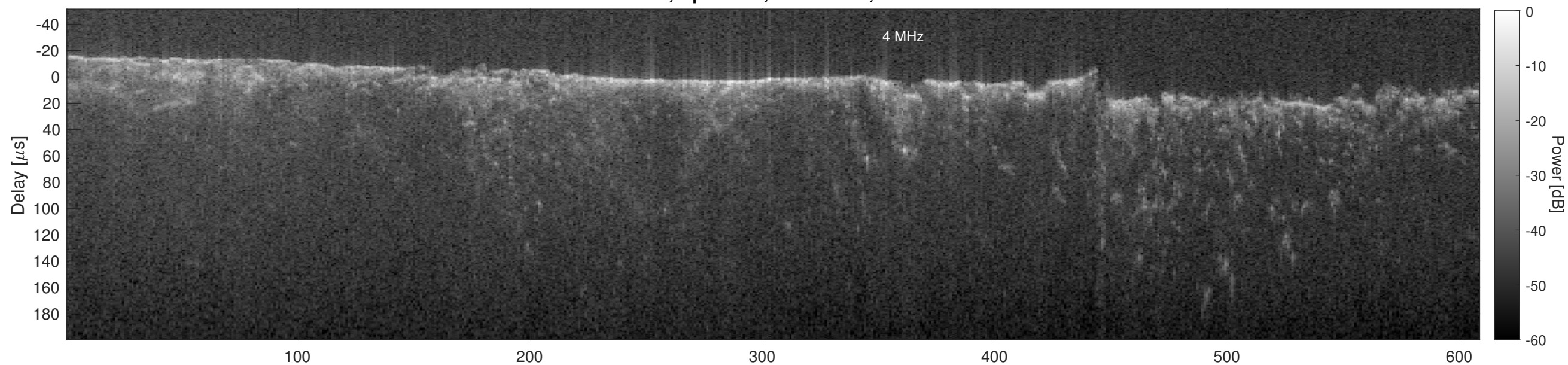
Orbit 6381, Cluttergram
