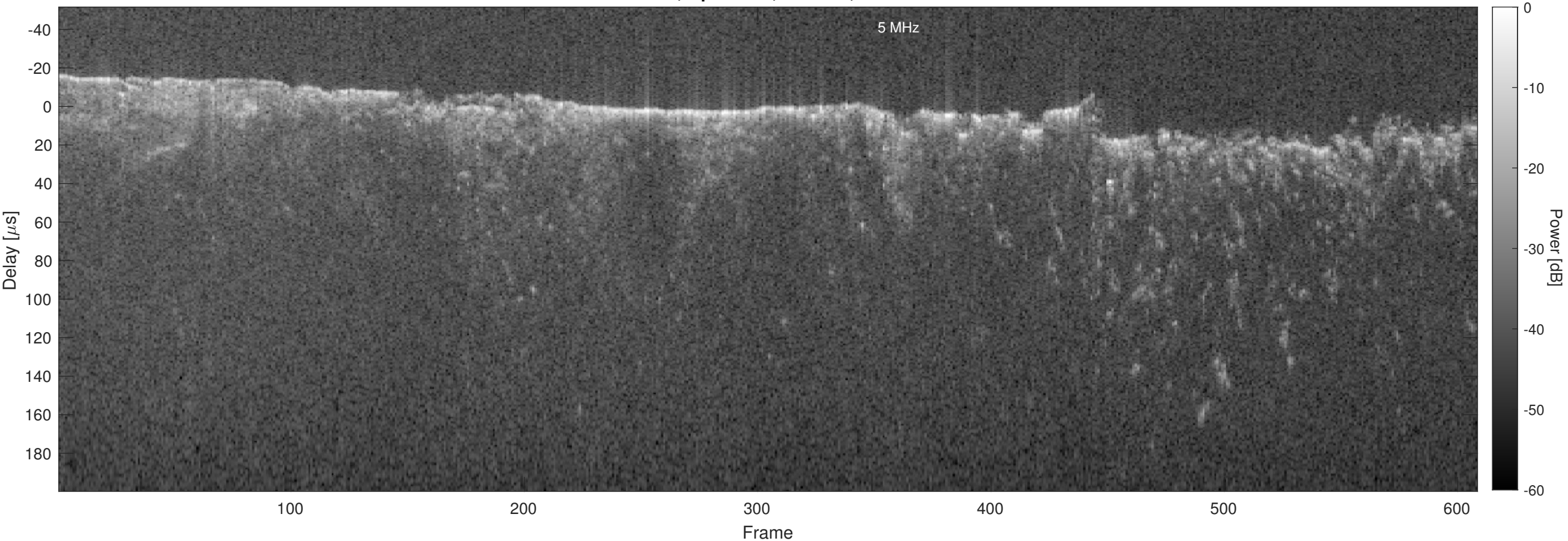
Orbit 6381, Optimized, Window, Channel 2
