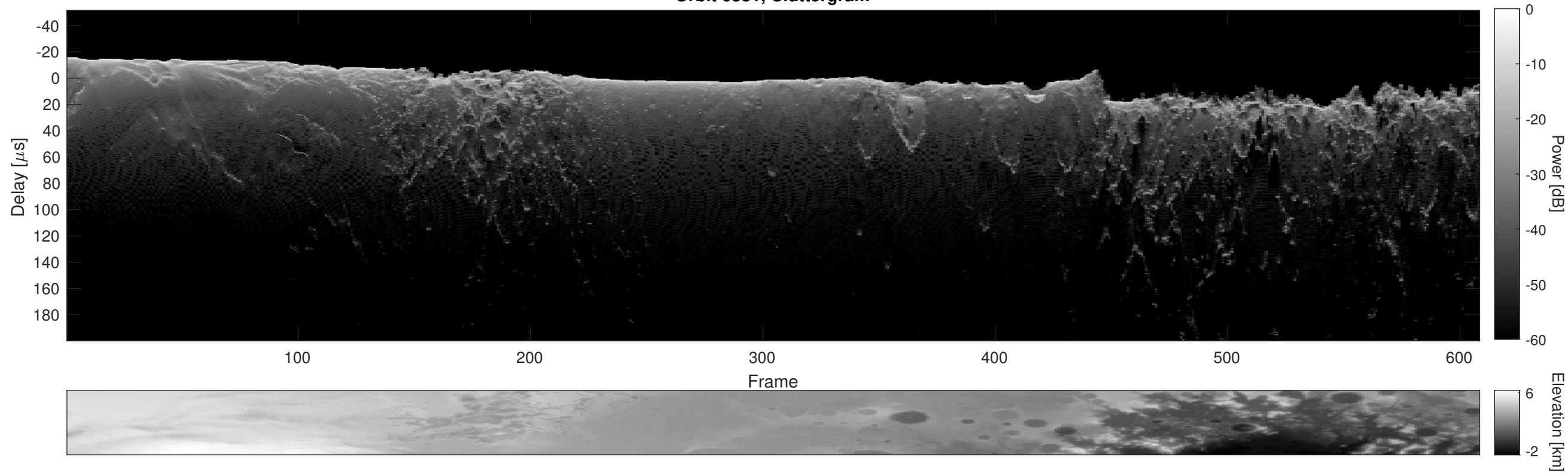
Orbit 6381, Cluttergram
