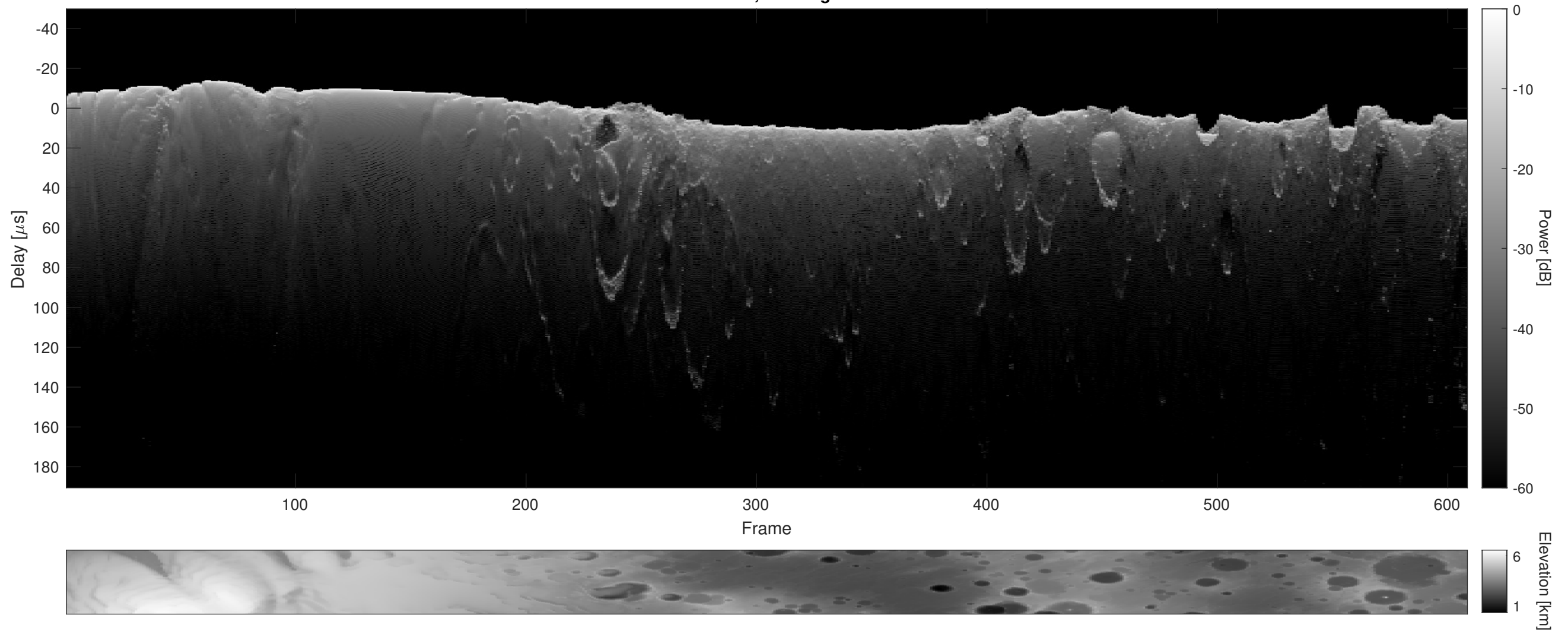
Orbit 6382, Cluttergram
