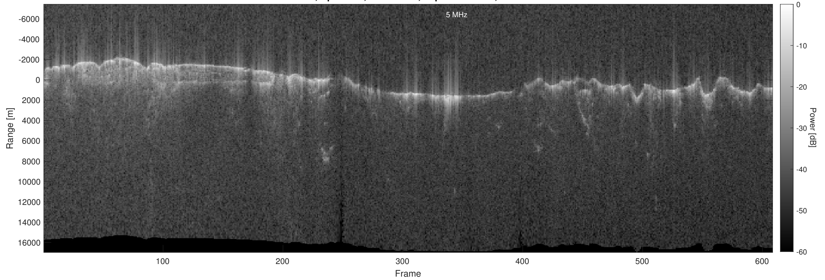
Orbit 6382, Optimized, No Window, Depth-Corrected, Channel 2
