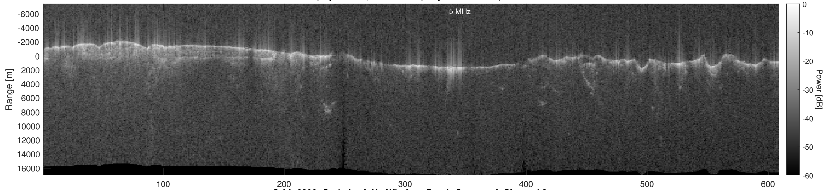
Orbit 6382, Optimized, No Window, Depth-Corrected, Channel 2
