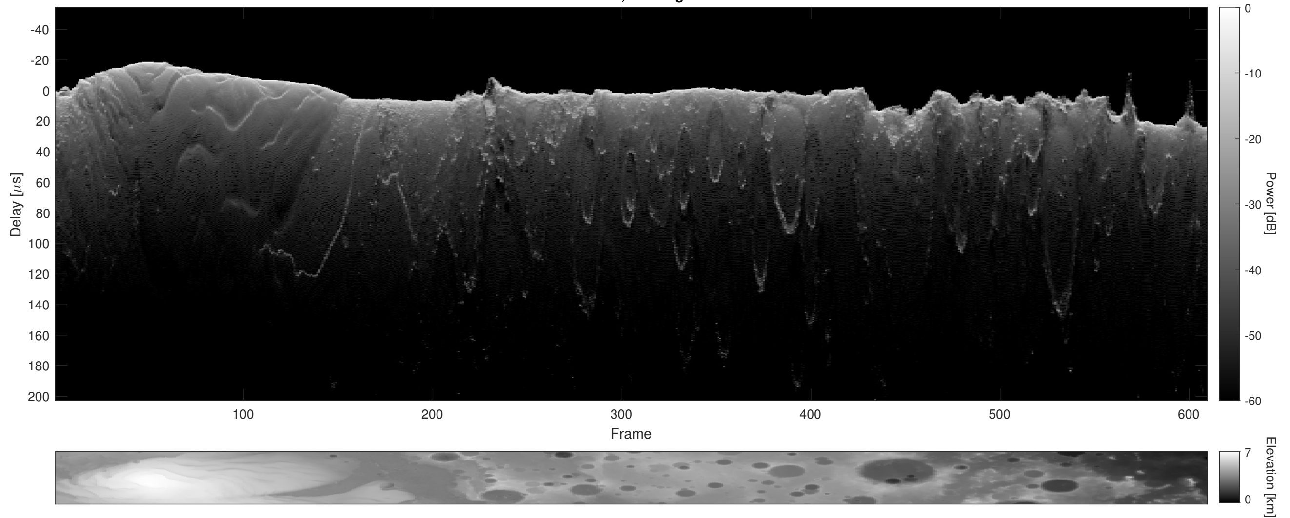
Orbit 6383, Cluttergram
