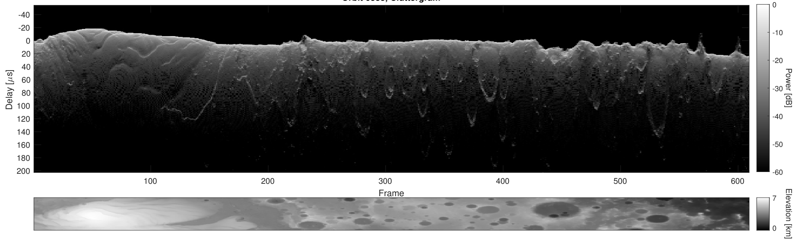
Orbit 6383, Cluttergram
