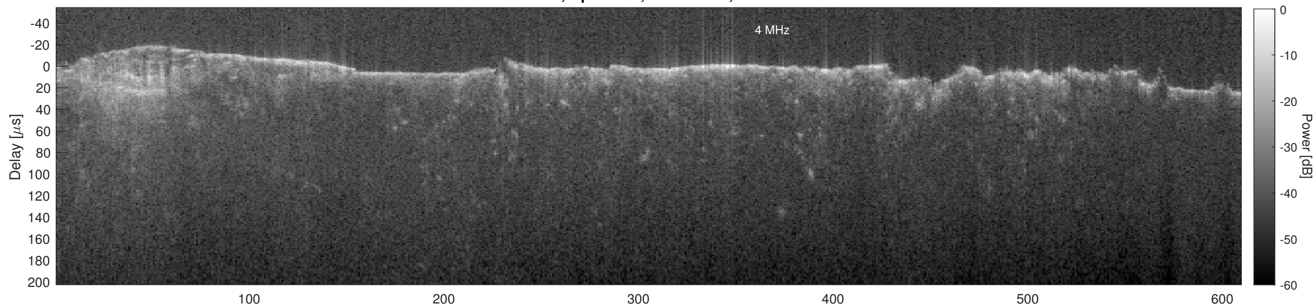
Orbit 6383, Cluttergram
