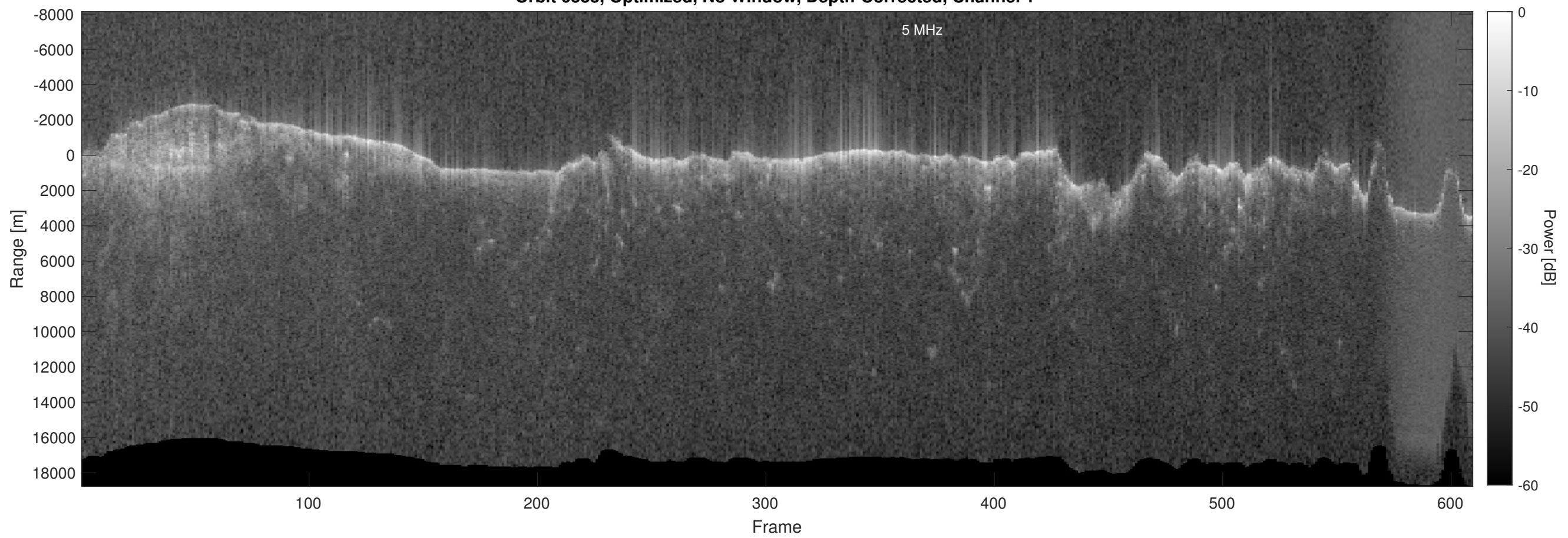
Orbit 6383, Optimized, No Window, Depth-Corrected, Channel 2
