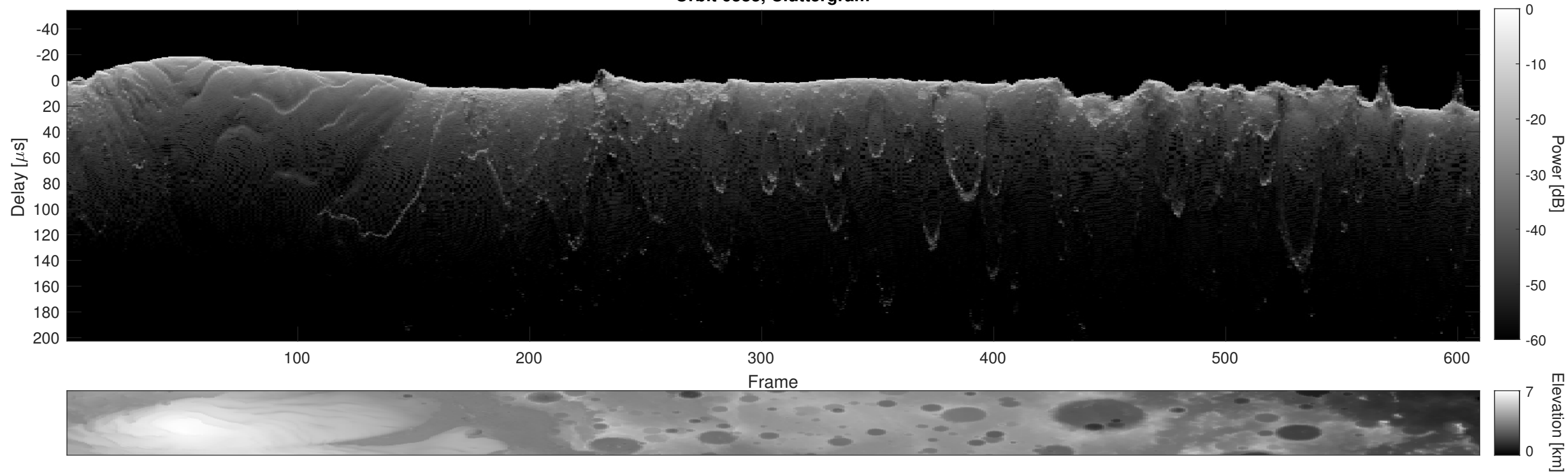
Orbit 6383, Cluttergram
