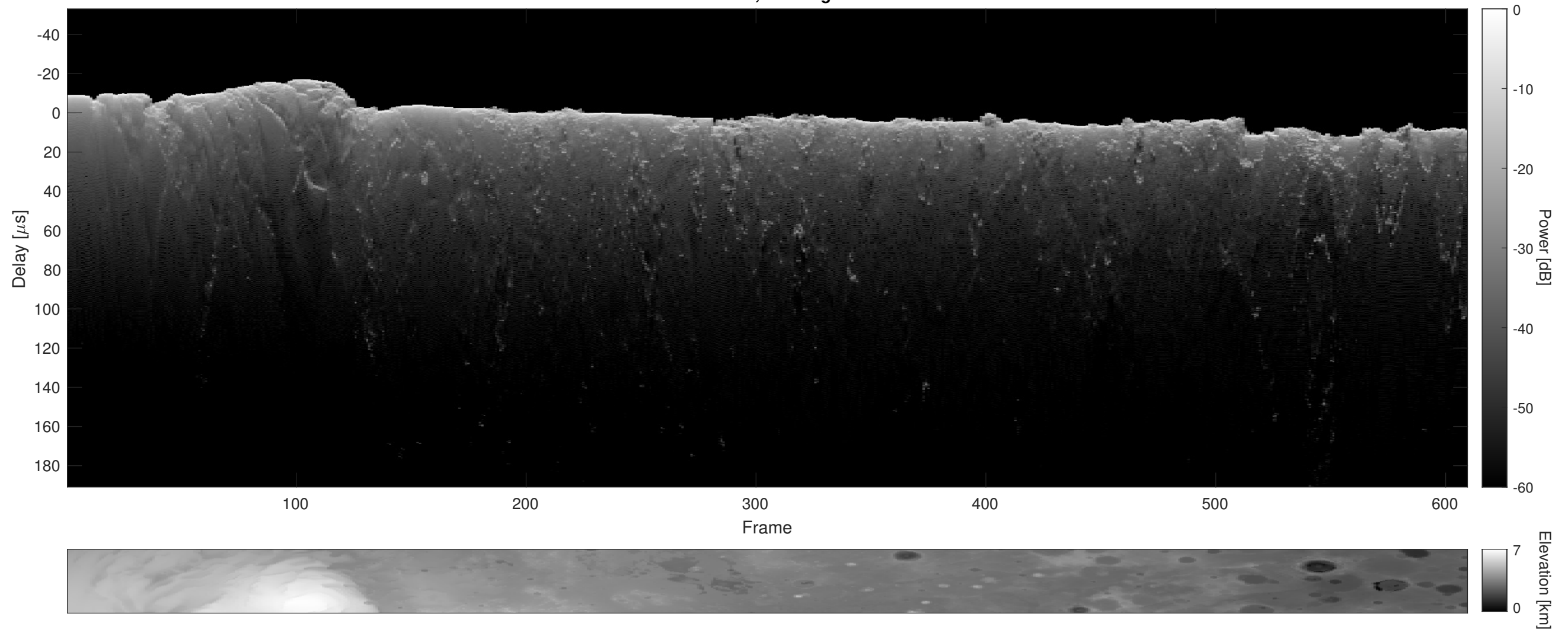
Orbit 6384, Cluttergram
