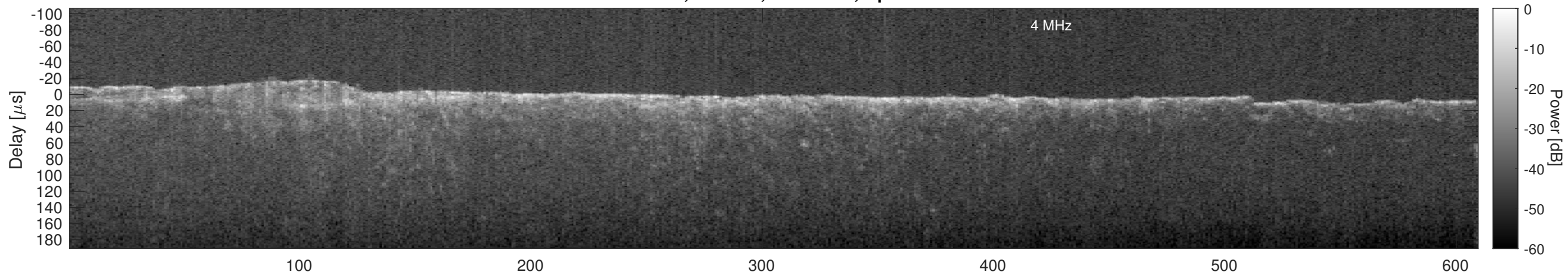
Orbit 6384, Cluttergram
