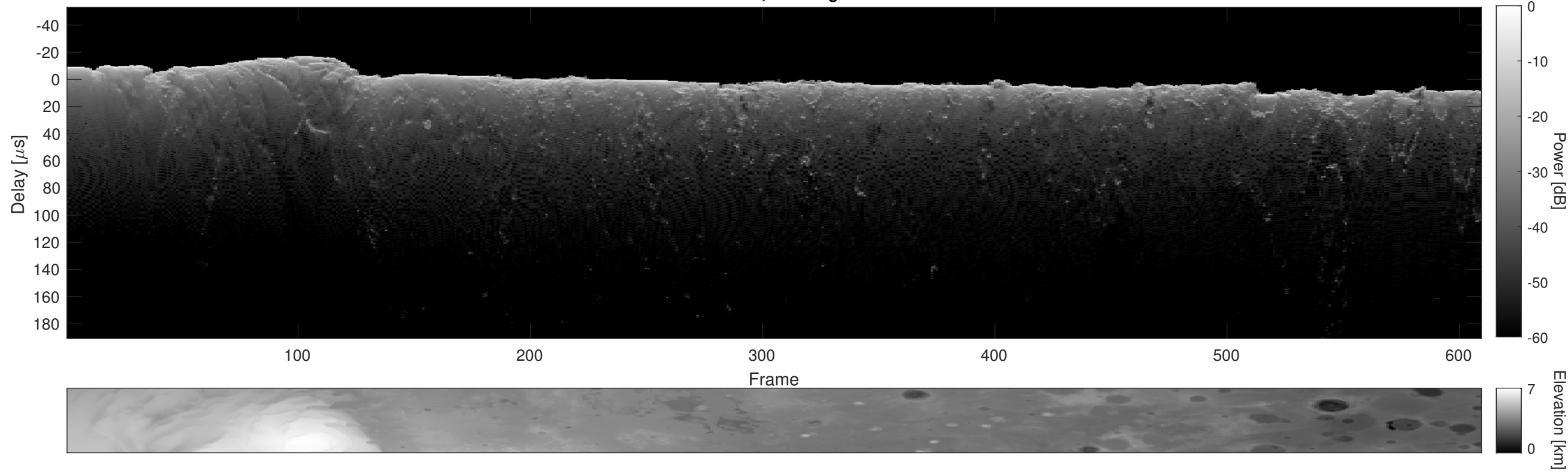
Orbit 6384, Cluttergram
