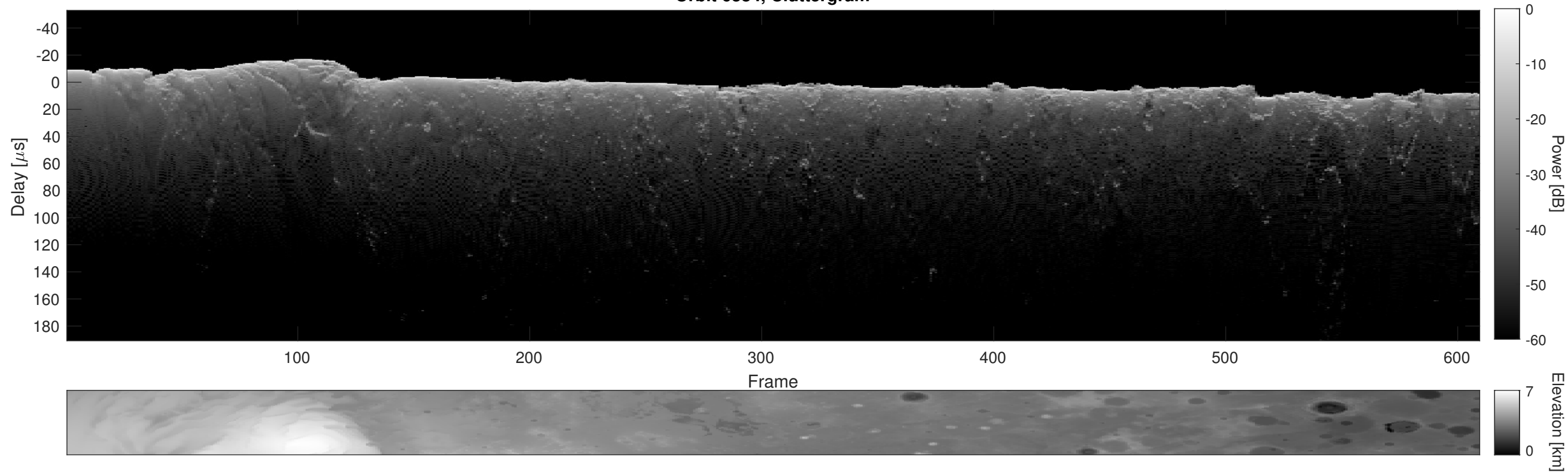
Orbit 6384, Cluttergram
