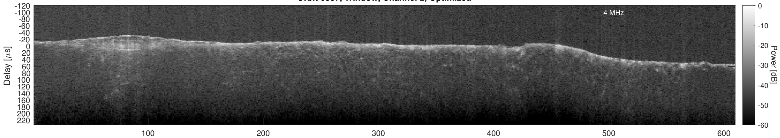
Orbit 6387, Cluttergram
