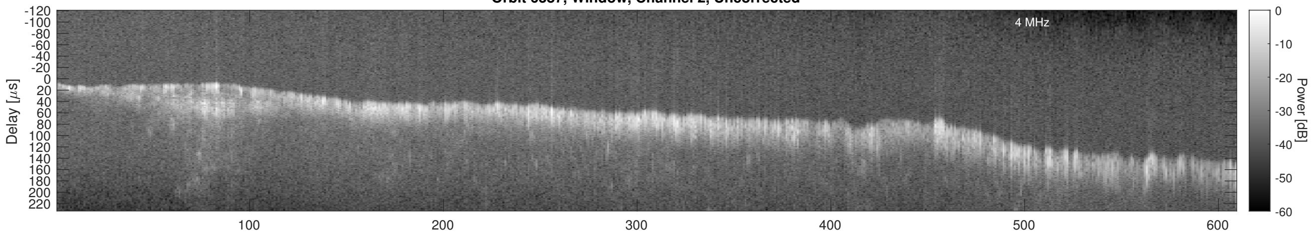
Orbit 6387, Window, Channel 2, Chapman
