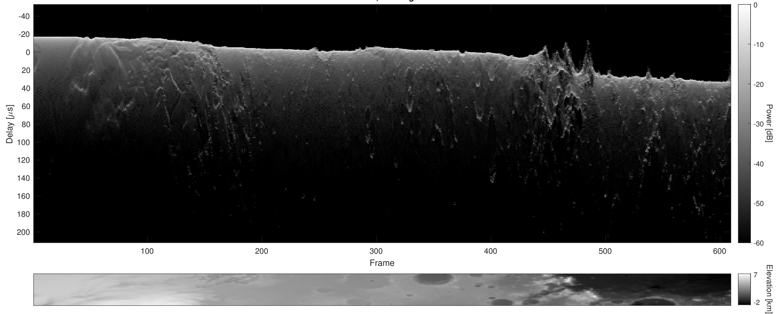
Orbit 6388, Cluttergram
