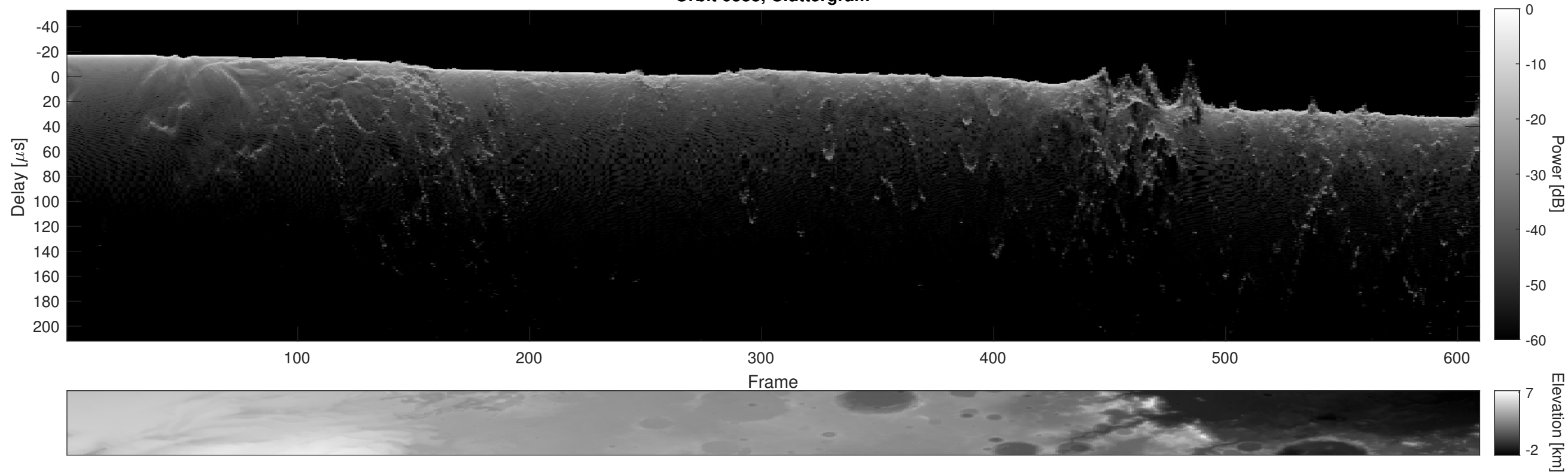
Orbit 6388, Cluttergram
