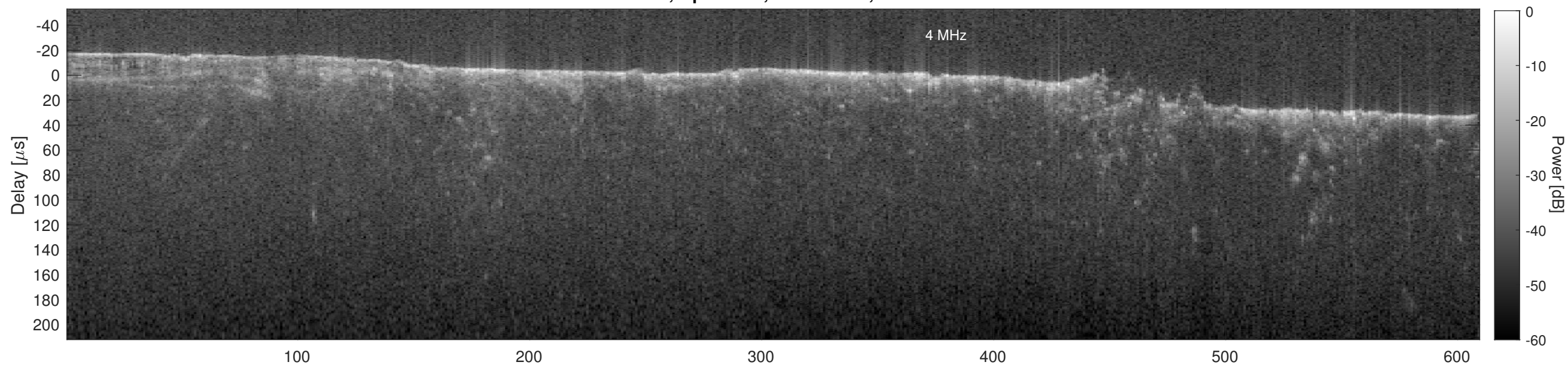
Orbit 6388, Cluttergram
