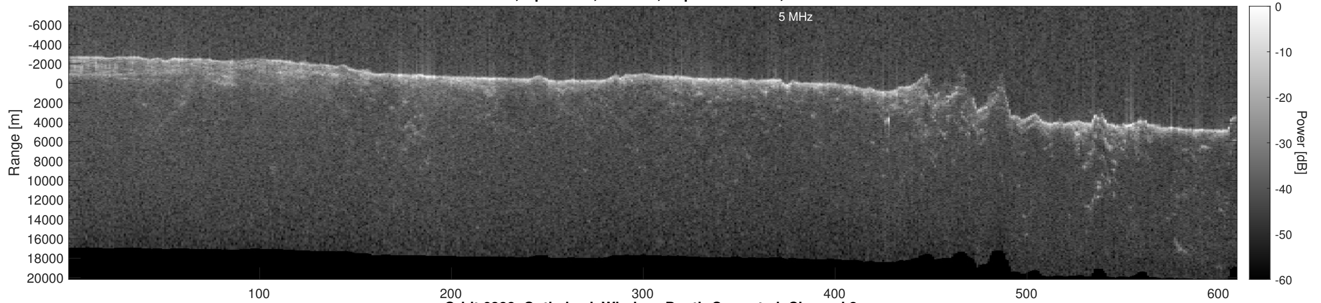
Orbit 6388, Optimized, Window, Depth-Corrected, Channel 2
