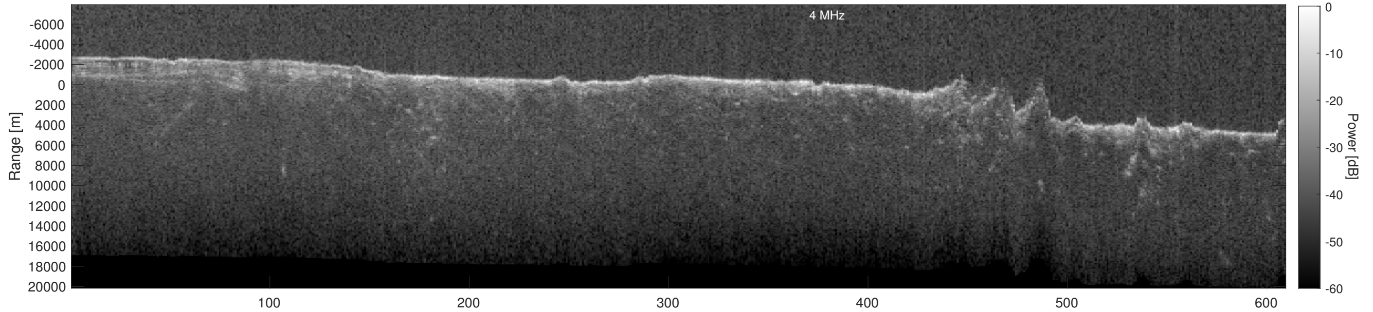
Orbit 6388, Depth-Corrected Cluttergram
