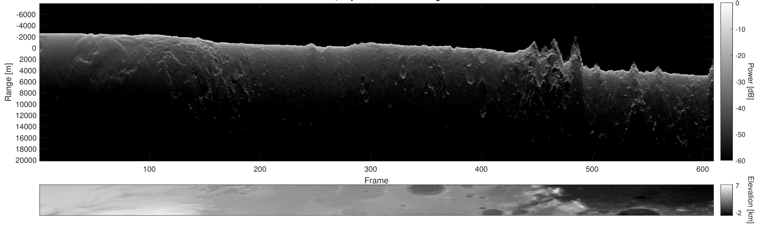
Orbit 6388, Depth-Corrected Cluttergram
