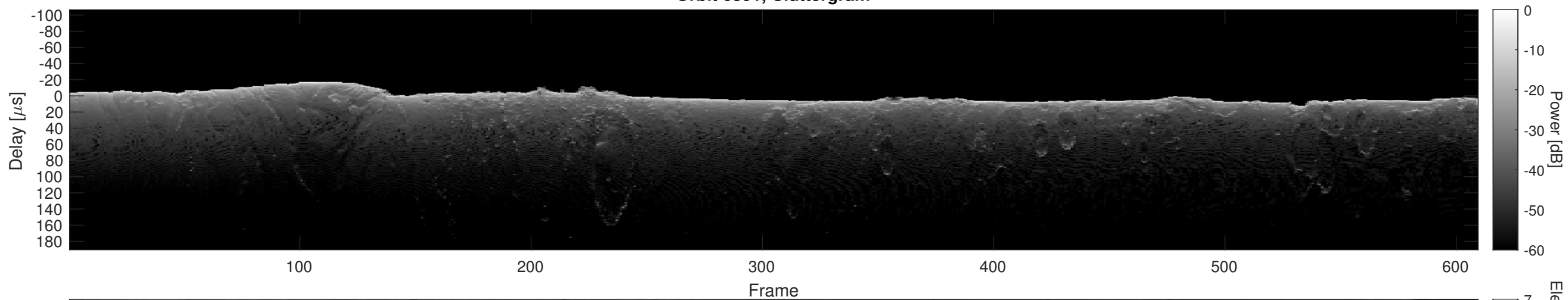
Orbit 6391, Cluttergram
