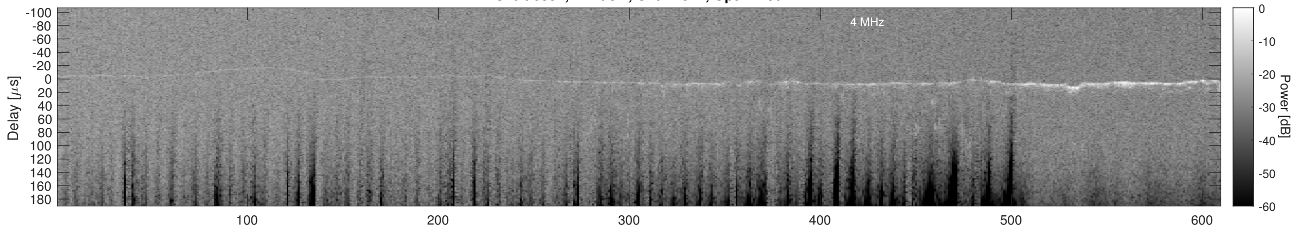
Orbit 6391, Cluttergram
