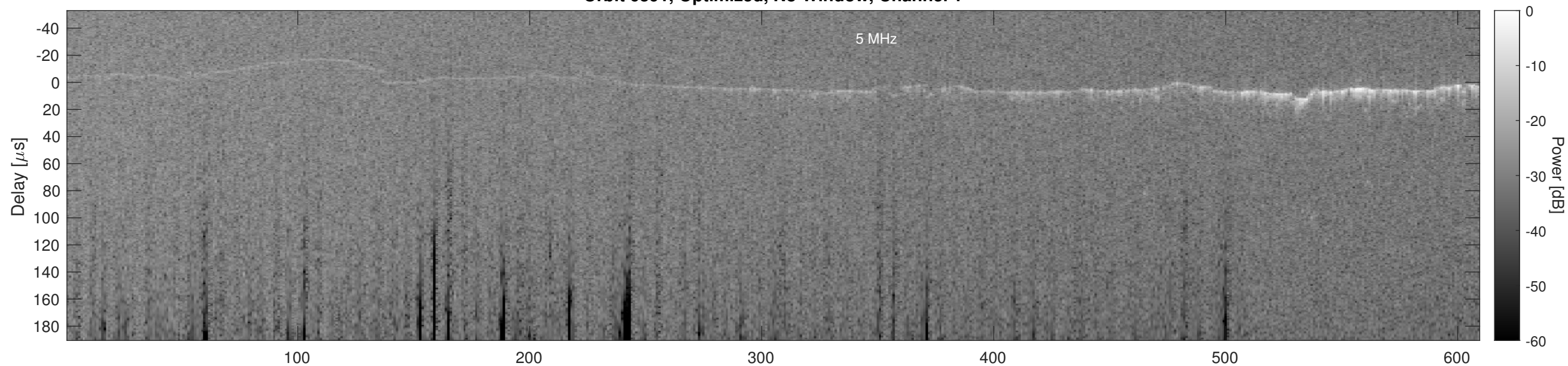
Orbit 6391, Optimized, No Window, Channel 2
