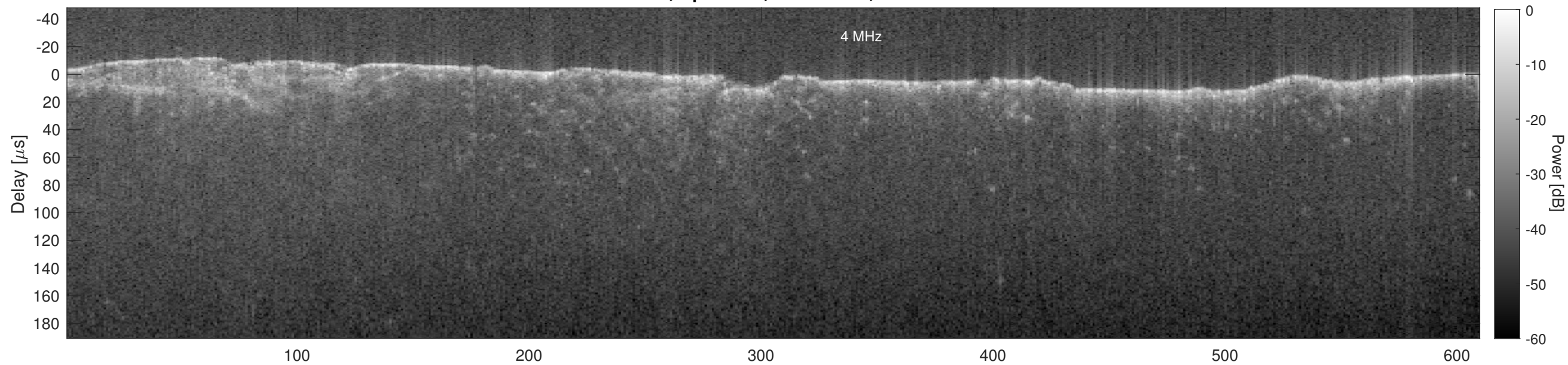
Orbit 6392, Cluttergram
