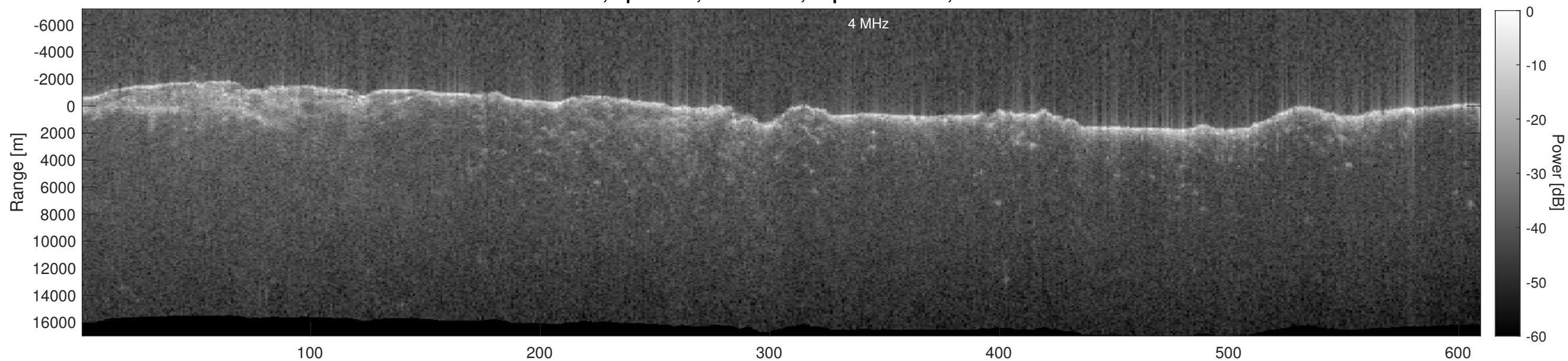
Orbit 6392, Depth-Corrected Cluttergram
