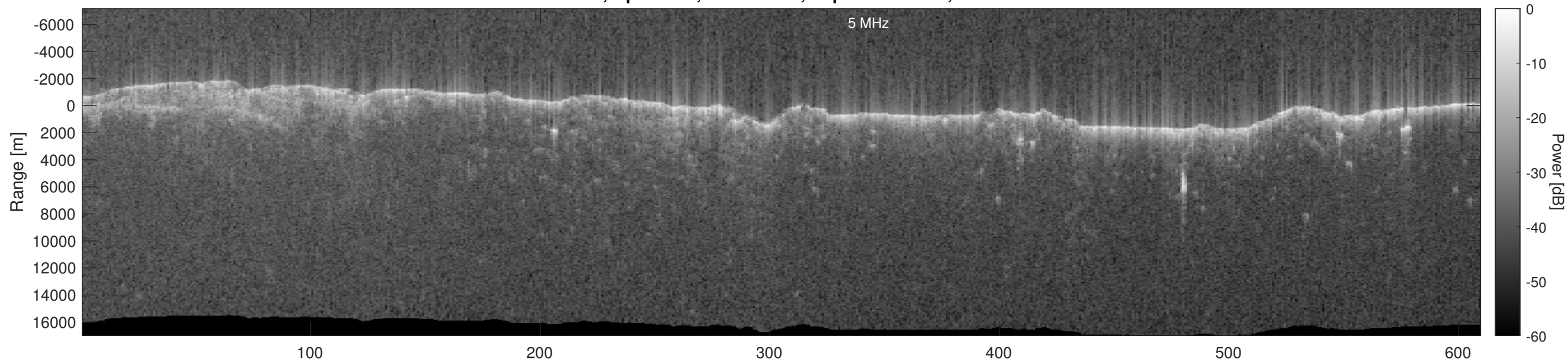
Orbit 6392, Optimized, No Window, Depth-Corrected, Channel 2
