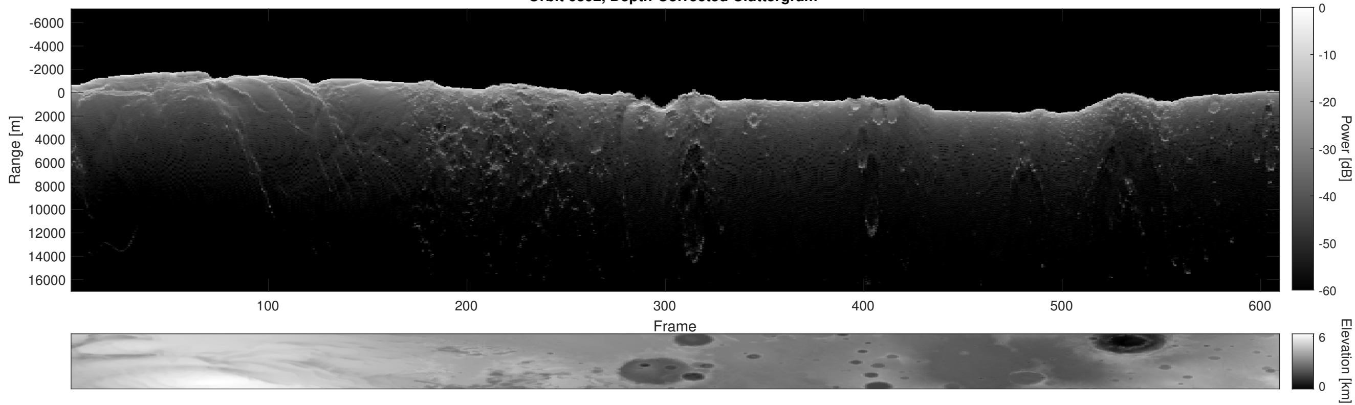
Orbit 6392, Depth-Corrected Cluttergram
