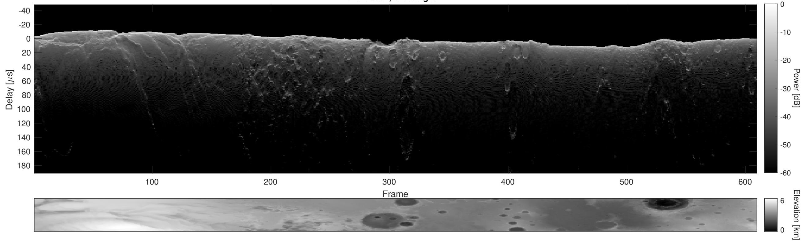
Orbit 6392, Cluttergram
