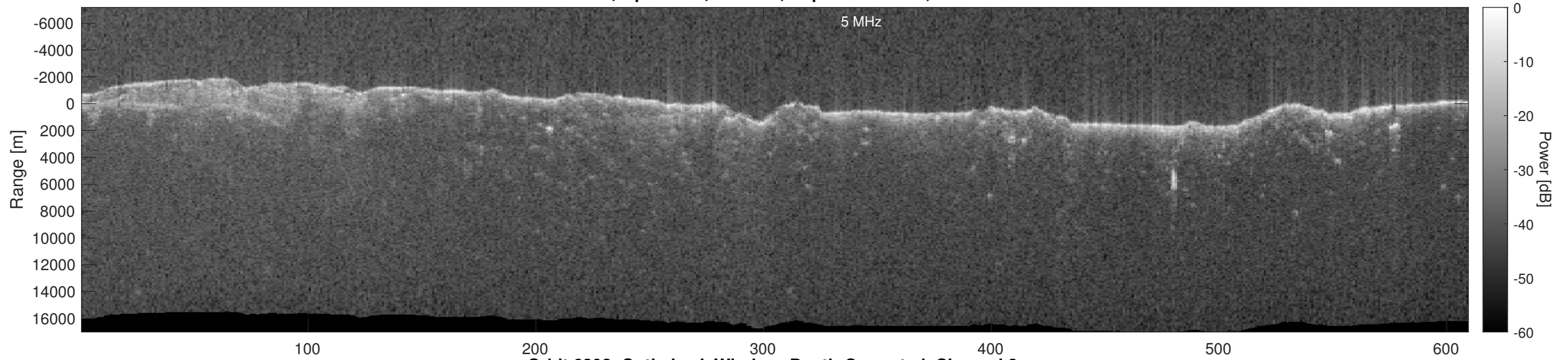
Orbit 6392, Optimized, Window, Depth-Corrected, Channel 2
